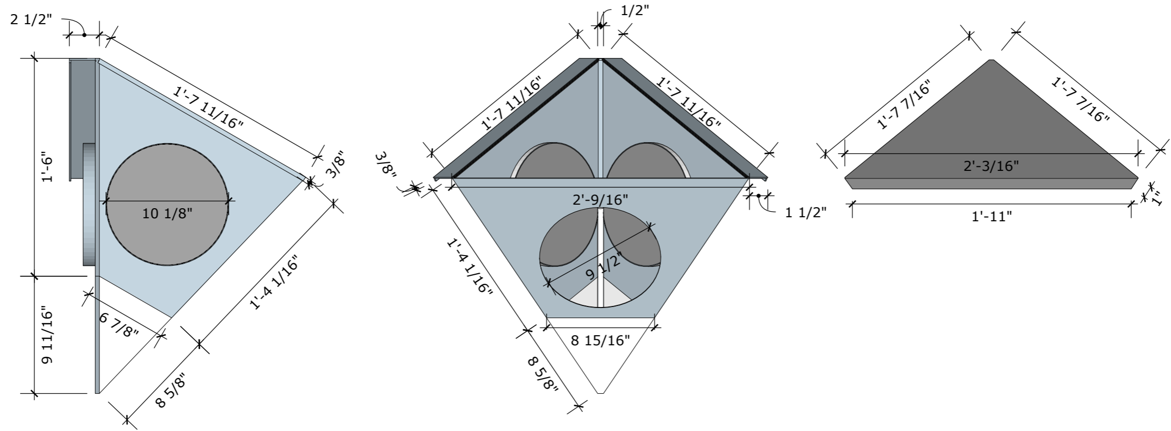
BUBBLE GENERATOR
