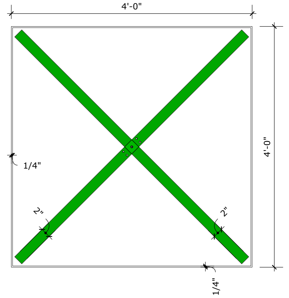
FLOOR PLAN
