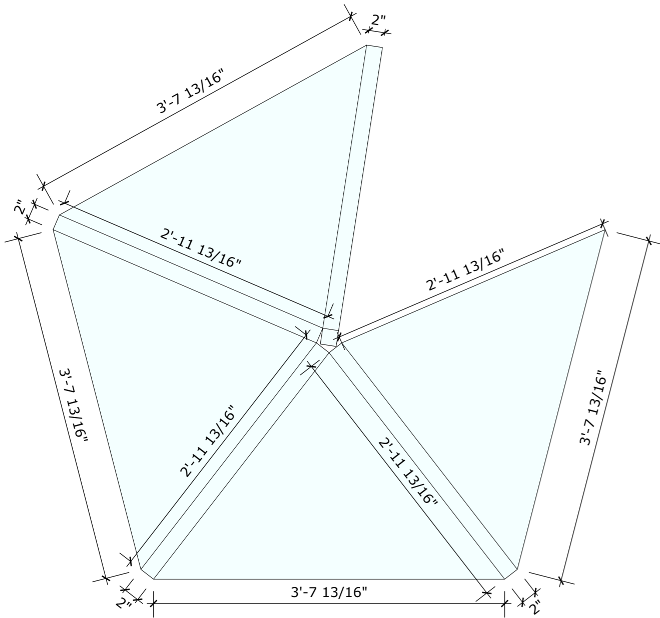
TOP PYRAMID EXPANSION VIEW
