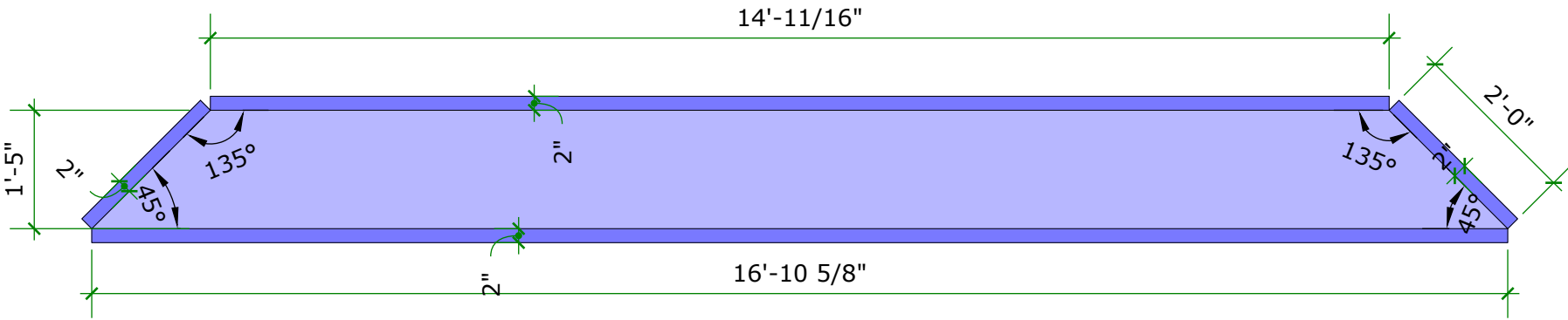
Bottom Piece x4
