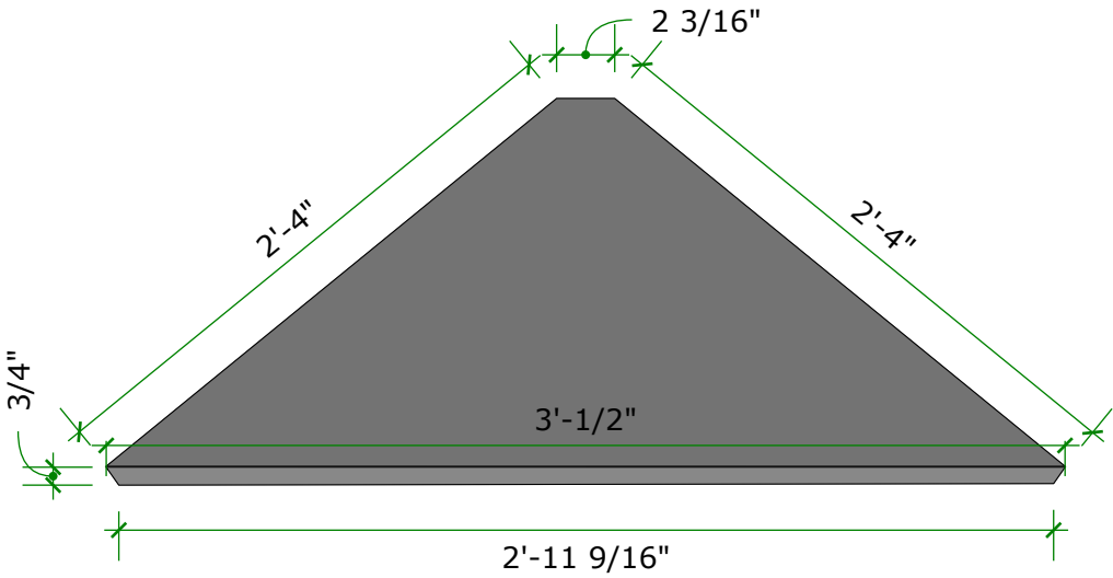
Sliding Top Cover
