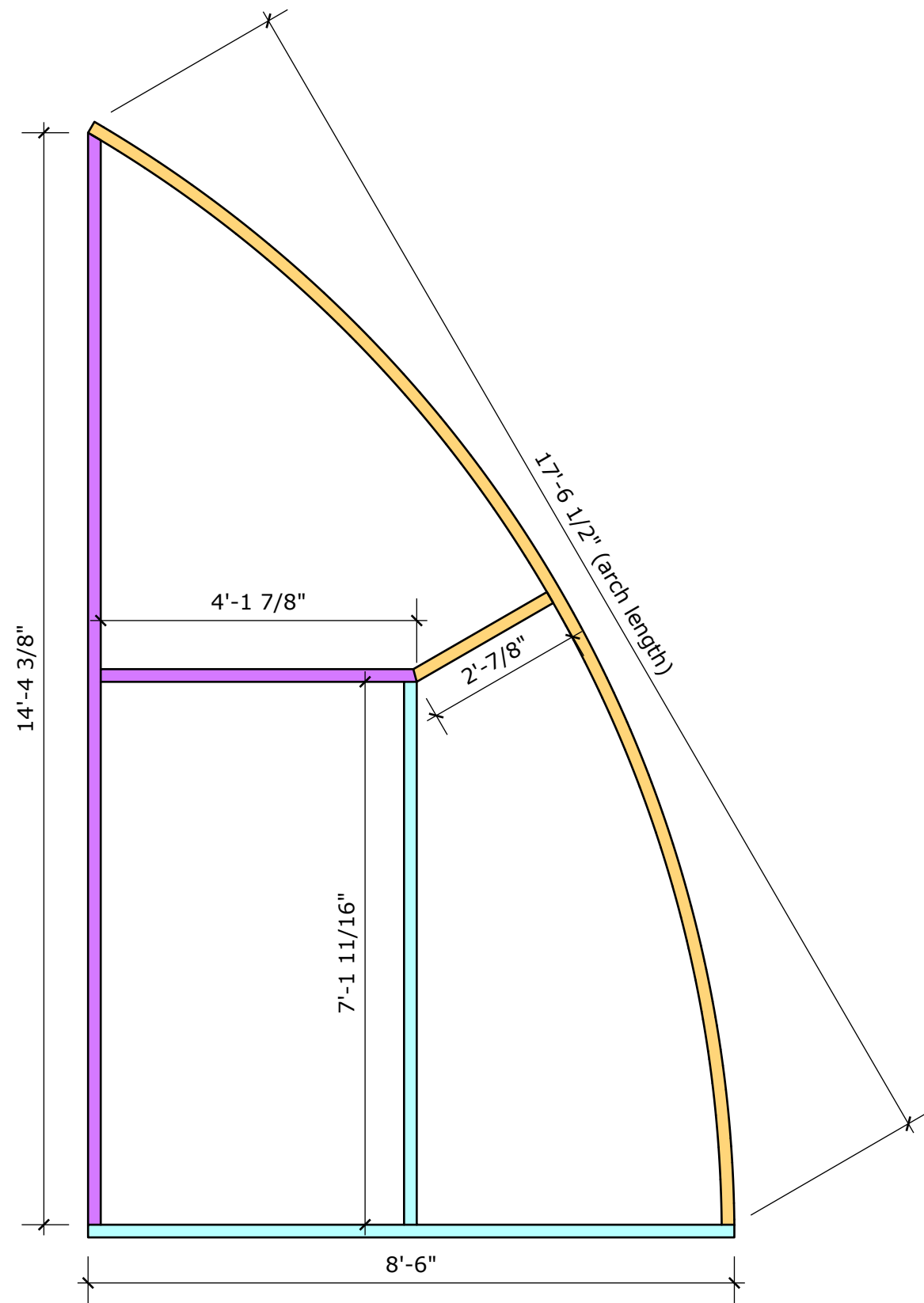
MAIN FRAME X1
